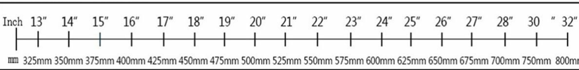
Image 6.1: International Wiper Size Chart (Inches and Millimeters).
