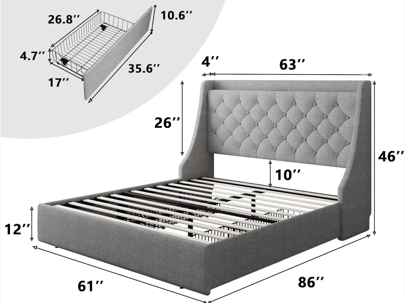
Image 8.1: Dimensional drawing of the iPormis Queen Bed Frame, including headboard height, frame length, and width.
