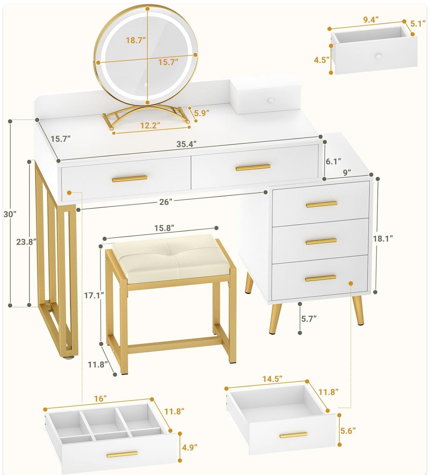
Figure 5: Detailed diagram showing the dimensions of the vanity desk, mirror, stool, and drawers.
