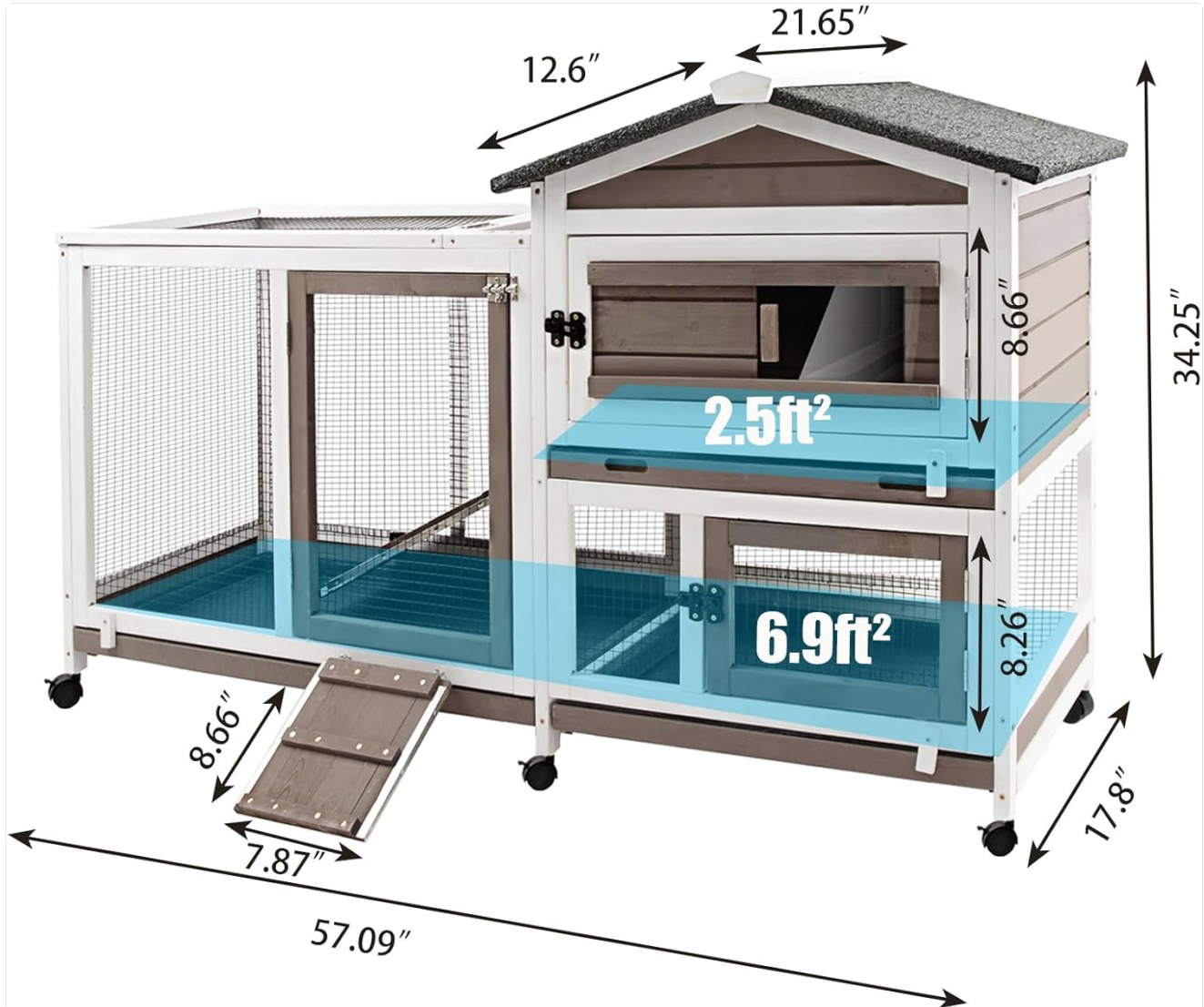
Image 8.1: Detailed dimensions of the PetsCosset Rabbit Hutch, including overall length, width, height, and internal area measurements for both levels.
