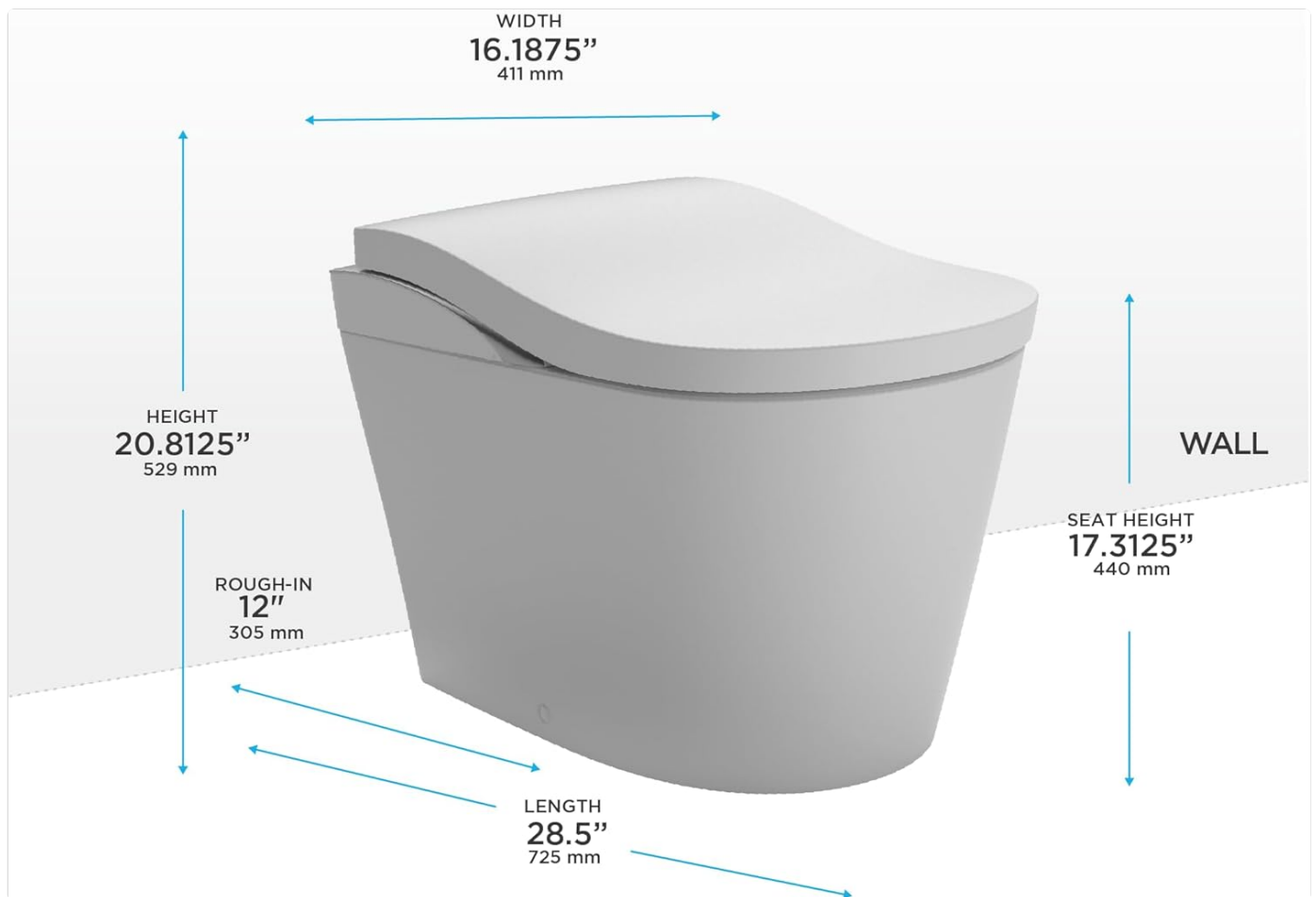
Image 2.1: Dimensional drawing of the TOTO Neorest LS toilet. This image provides key measurements including height (20.8125 inches), width (16.1875 inches), length (28.5 inches), seat height (17.3125 inches), and rough-in (12 inches).
