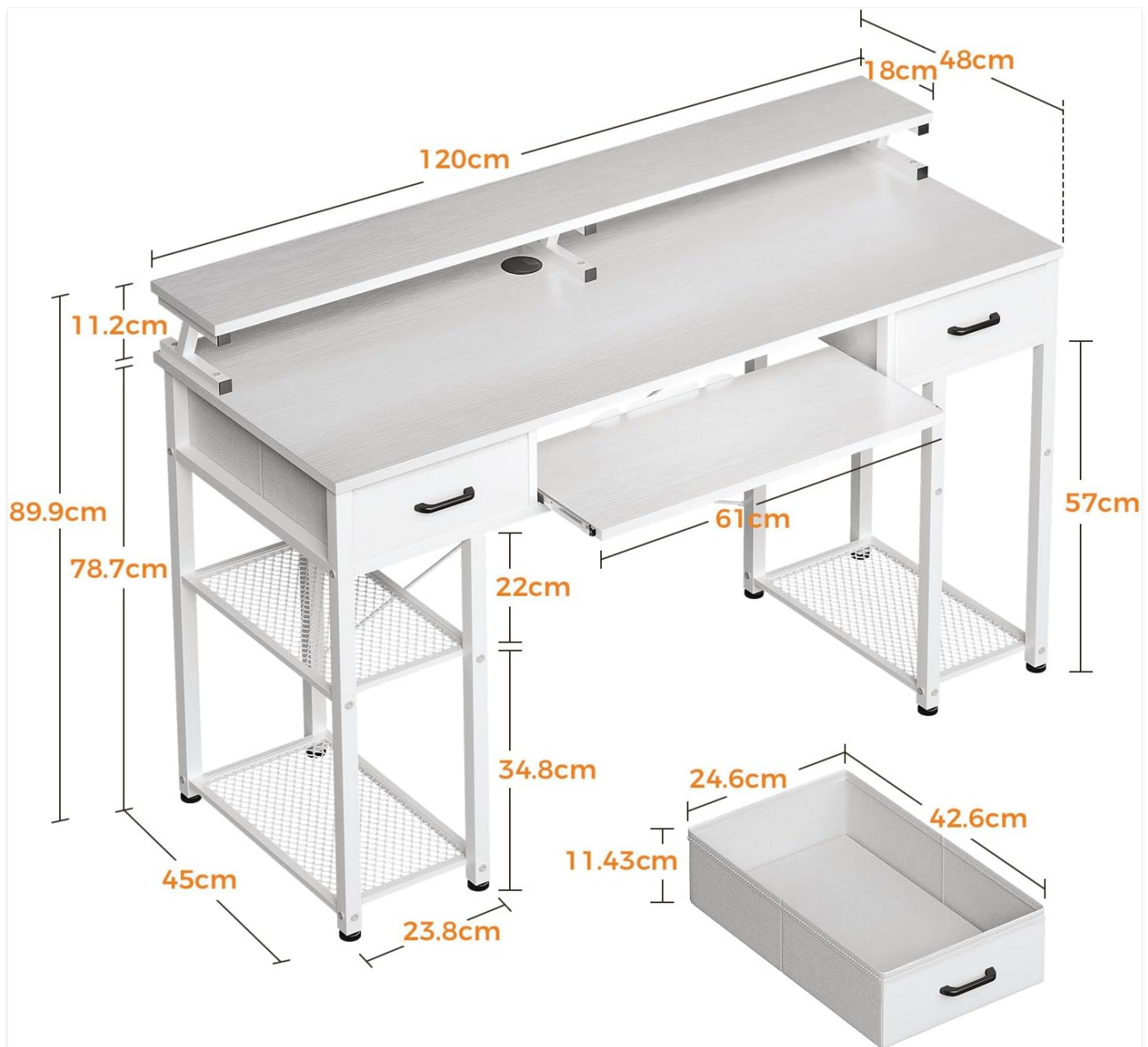
Figure 4.1: Comprehensive dimensions of the ODK Computer Desk, including overall height, width, depth, and specific measurements for shelves, keyboard tray, and drawers.
