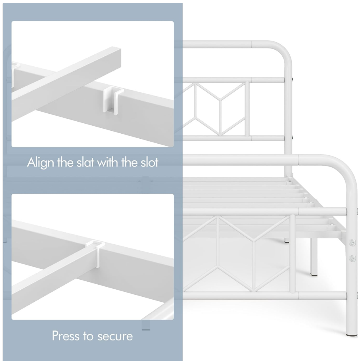
Image: Steps for aligning and securing the bed slats.
