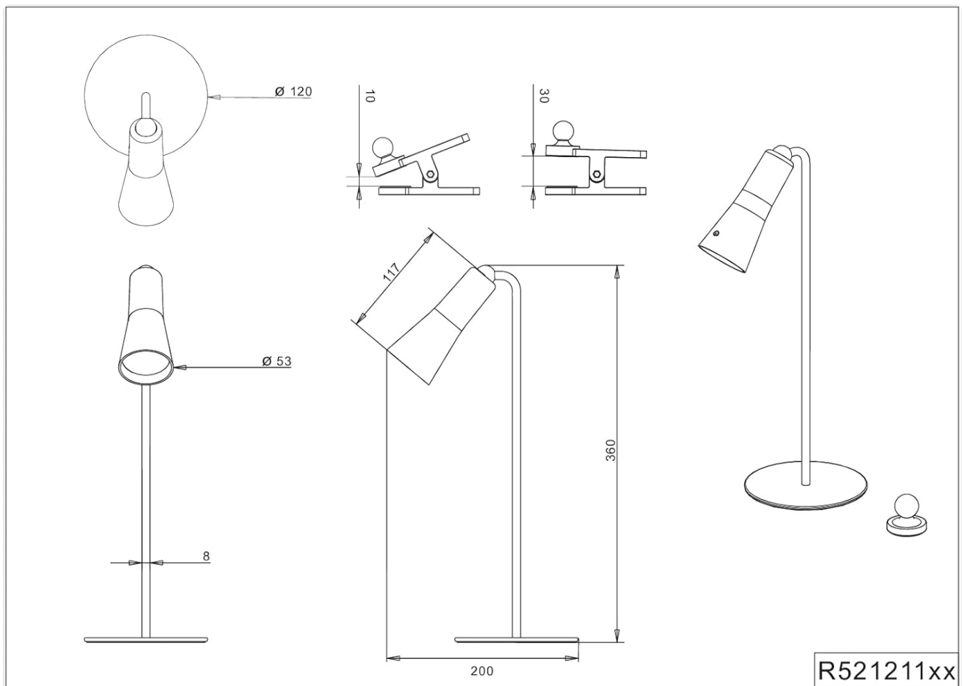
Image 8.1: Detailed technical drawing showing the dimensions of the lamp and its components in millimeters.
