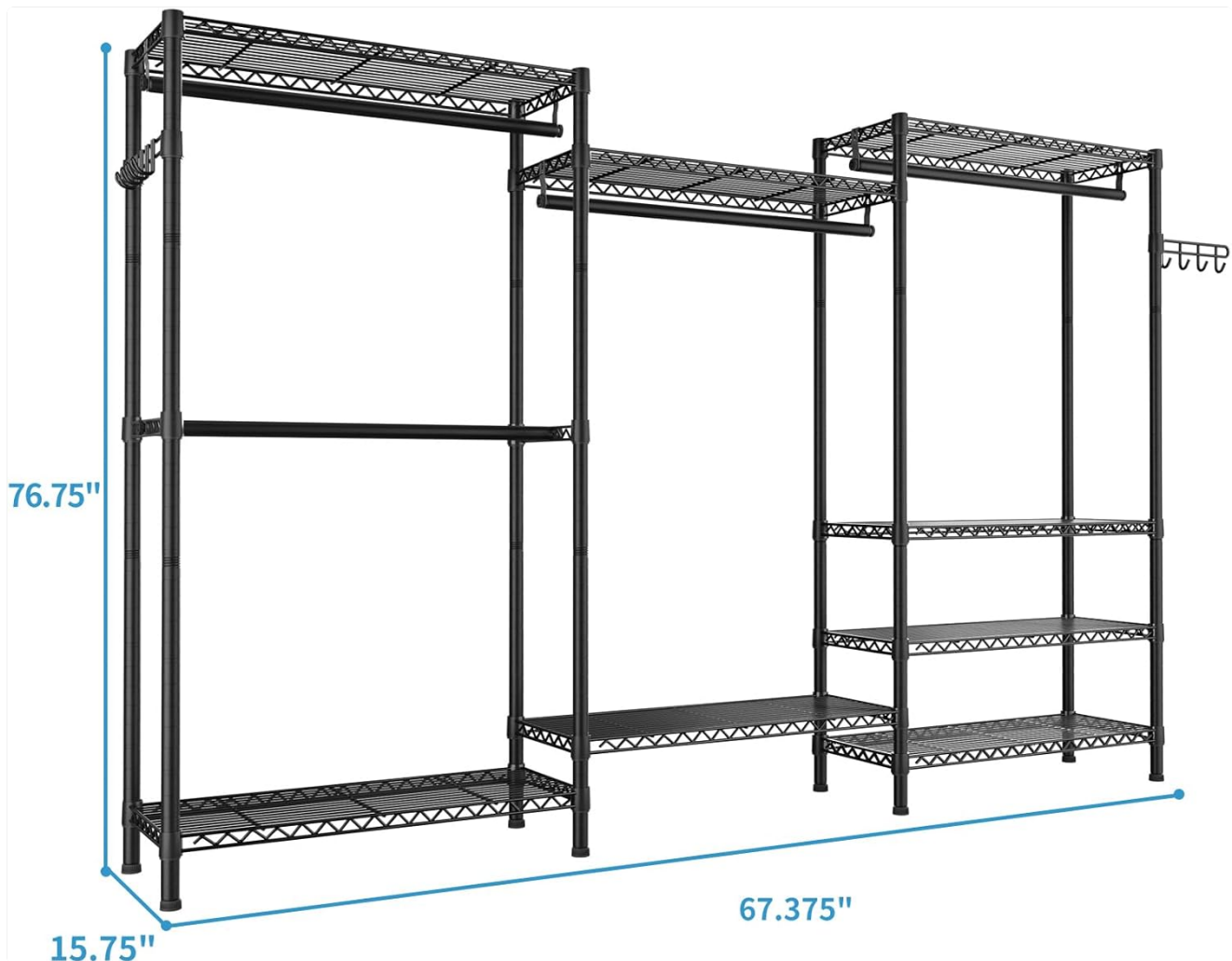
Image 7.1: Dimensional overview of the Golpart Heavy Duty Garment Rack.
