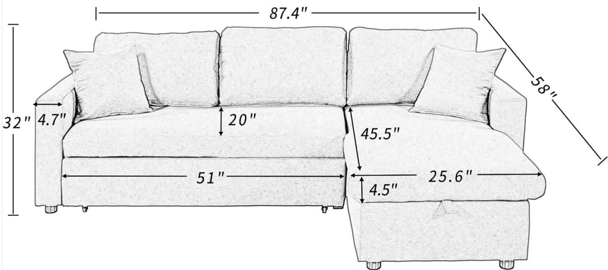
Image 8.1: Detailed dimensions of the sofa bed.
