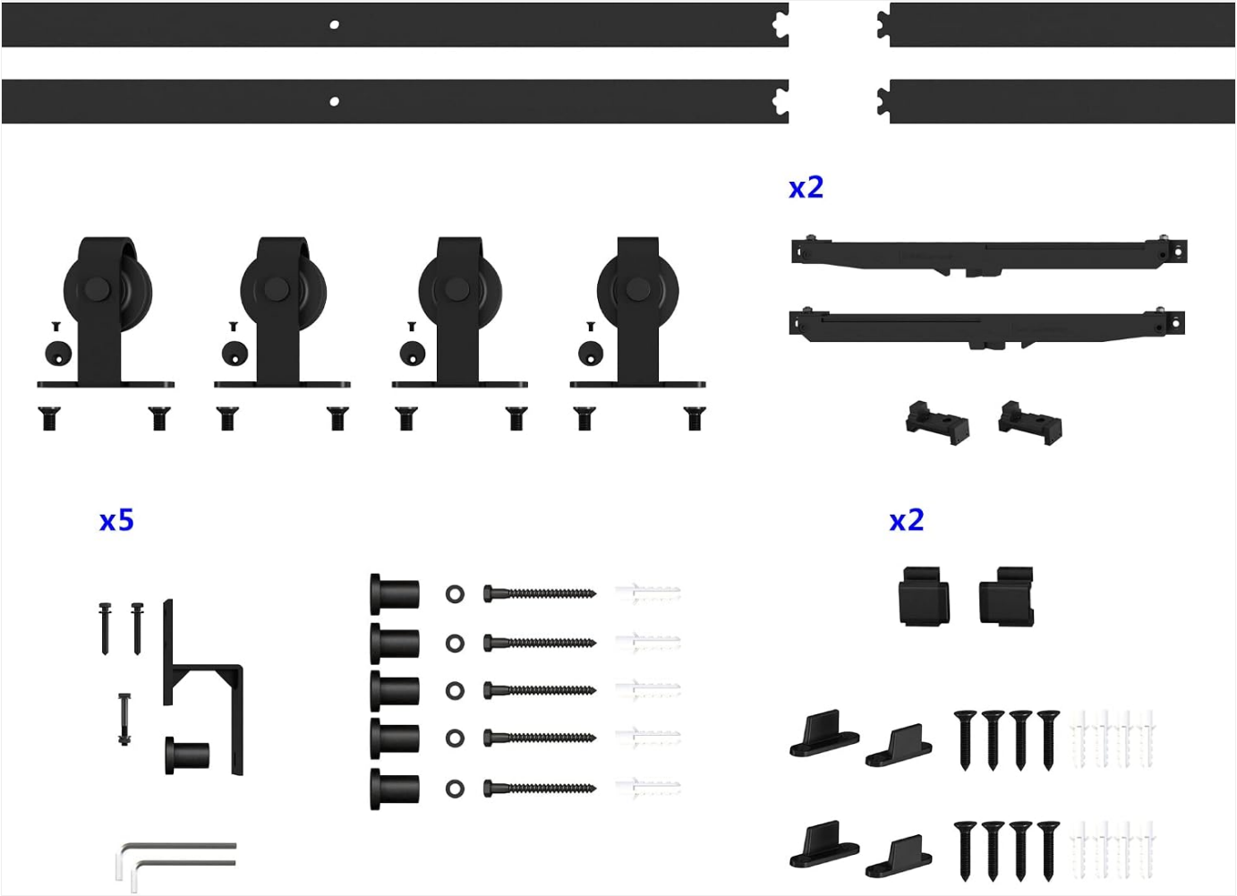
Image: An illustration showing all the hardware components included in the JUBEST Bypass Glass Barn Door kit, such as rails, rollers, soft-close mechanisms, and mounting accessories.
