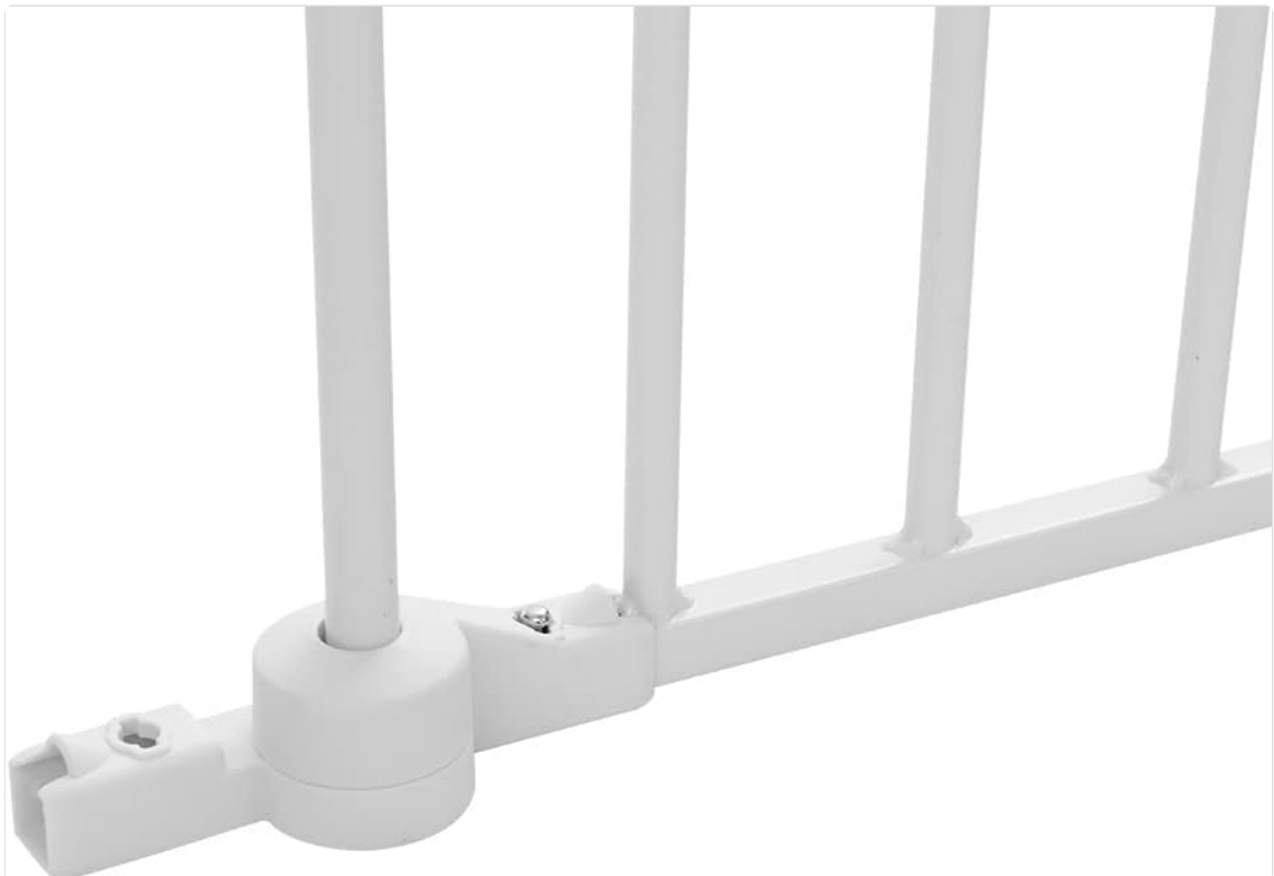
Image: Detail of the bottom connection point, showing the corresponding hole and spring clip for secure attachment.
