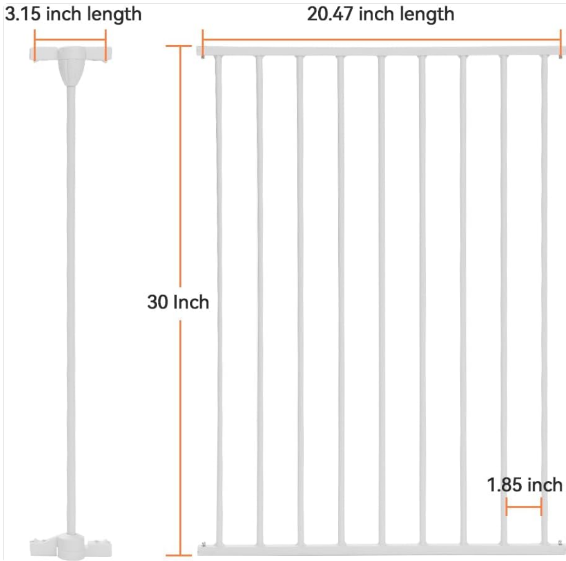
Image: The COMOMY Gate Extension panel with key dimensions: 30 inches tall, 20.47 inches length (panel width), 3.15 inches length (top connector), and 1.85 inches (bar spacing).
