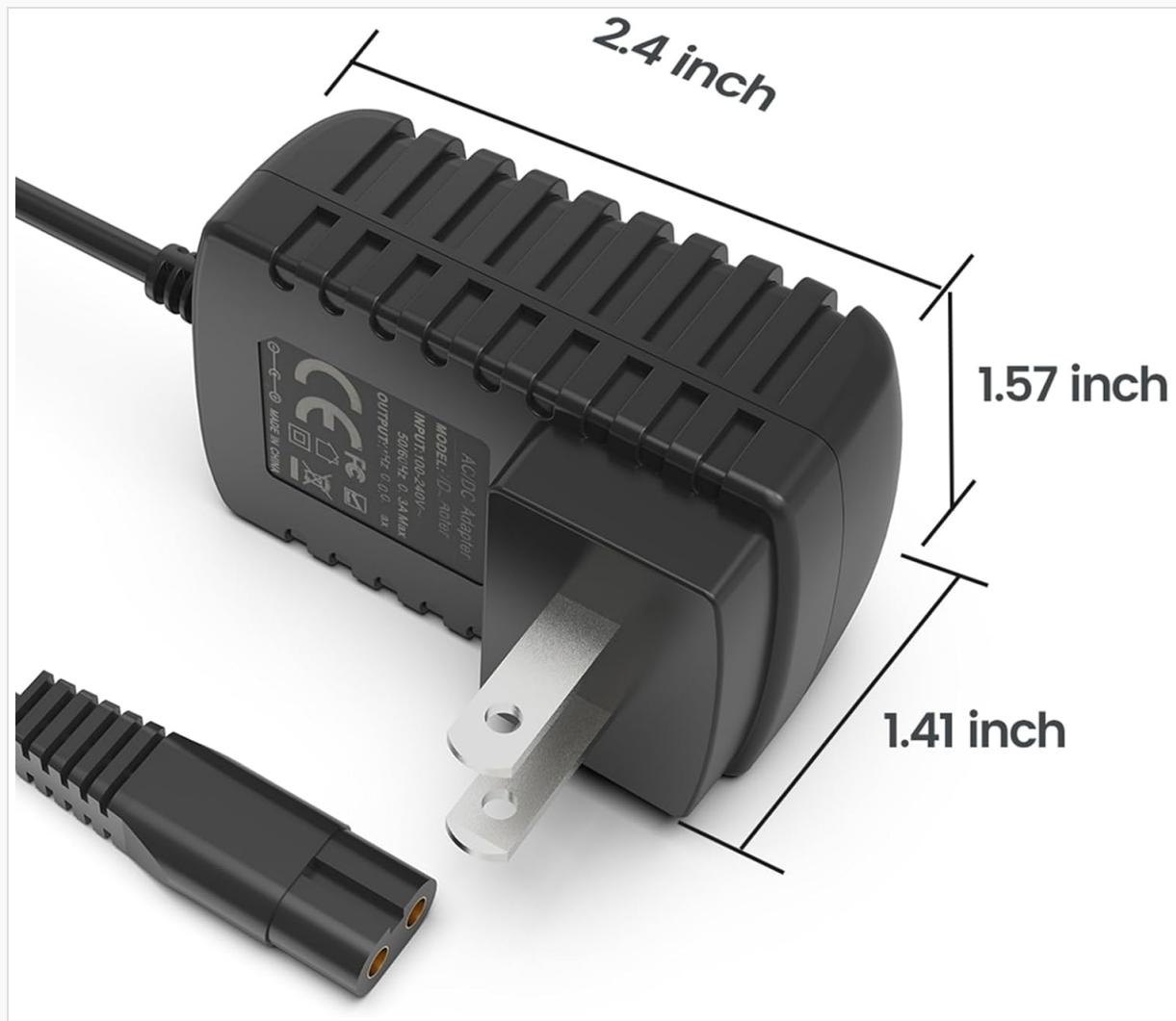
Image: The VOJSALDR D4.5V-1 charger with its physical dimensions indicated: 2.4 inches in length, 1.57 inches in width, and 1.41 inches in height.
