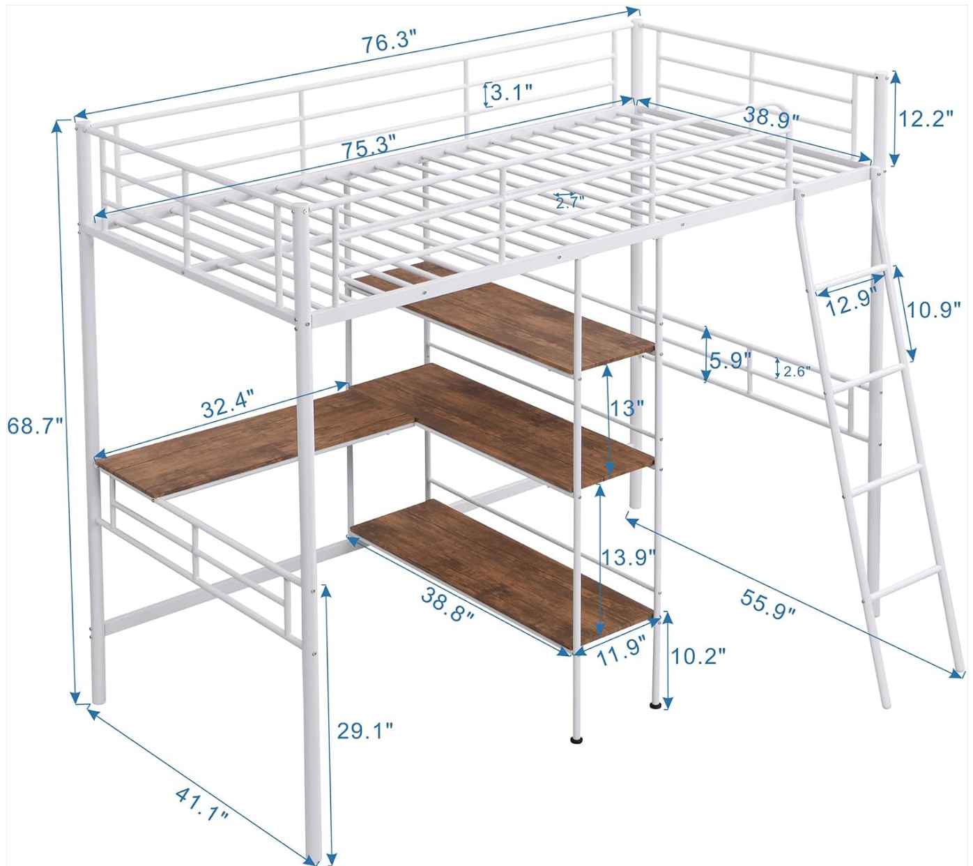
Figure 1: Detailed dimensions diagram of the Merax Metal Loft Bed, showing overall length, width, height, and individual component measurements for reference during assembly.
