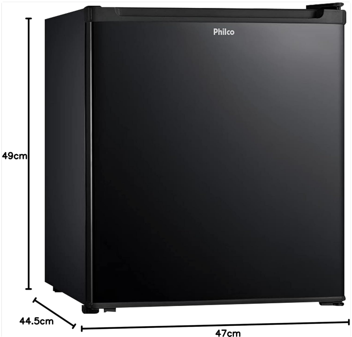
Figure 4.1: Dimensions of the Philco PFG50P Frigobar. The image displays the height (49cm), width (47cm), and depth (44.5cm) of the unit, crucial for proper placement.
