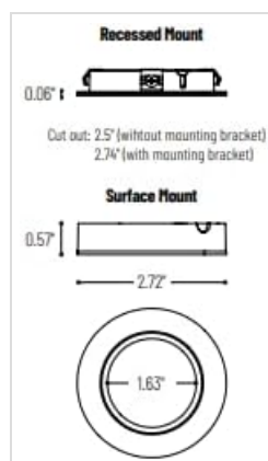
Figure 3: Detailed dimensional drawing illustrating the specifications for both recessed and surface mounting options. The recessed mount requires a 2.5-inch cutout (without mounting bracket) or 2.74-inch (with mounting bracket) and has a depth of 0.06 inches. The surface mount has a depth of 0.57 inches and a diameter of 2.72 inches.
