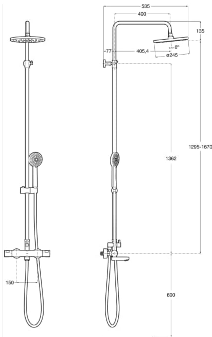
Figure 2: Technical drawing with key dimensions for installation.
