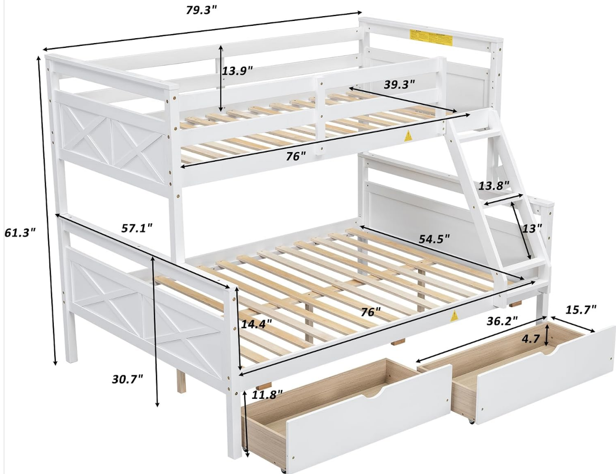
Image: Detailed dimensions diagram for the Merax Twin Over Full Bunk Bed.
