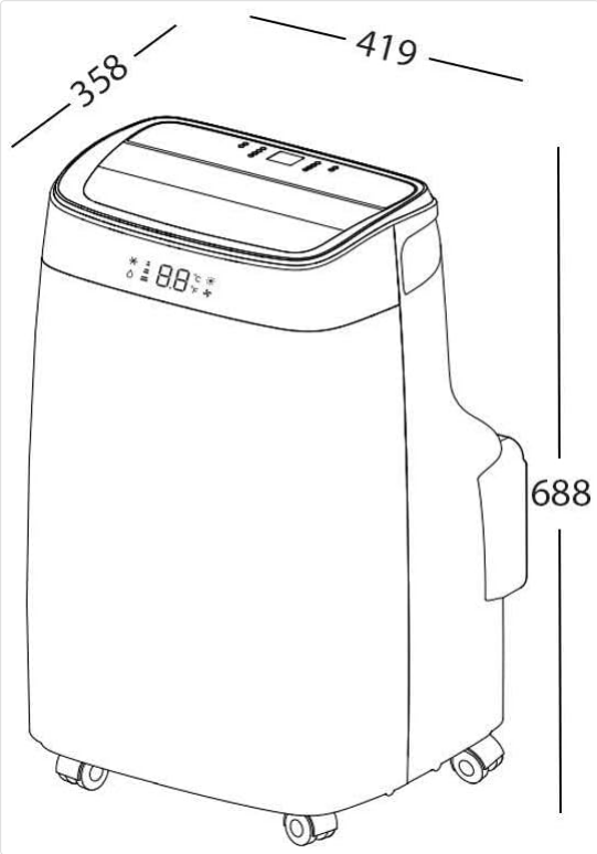
Figure 10.1: Dimensional drawing of the portable air conditioner.
