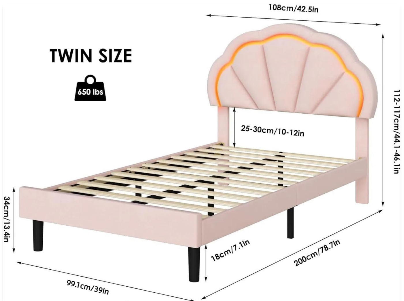
Image: An assembly diagram showing the dimensions of the Twin LED Bed Frame, including length, width, and adjustable headboard height, along with a 650 lbs weight capacity label.
