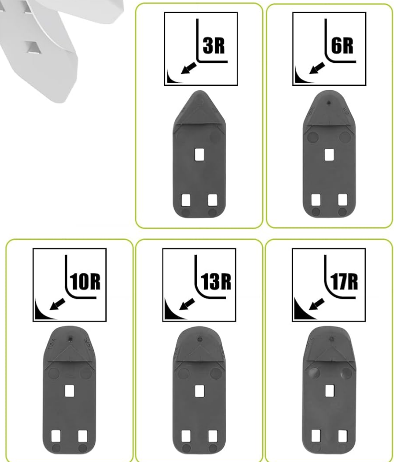
Image 3.2: The 5 replaceable silicone pads included with the tool.
