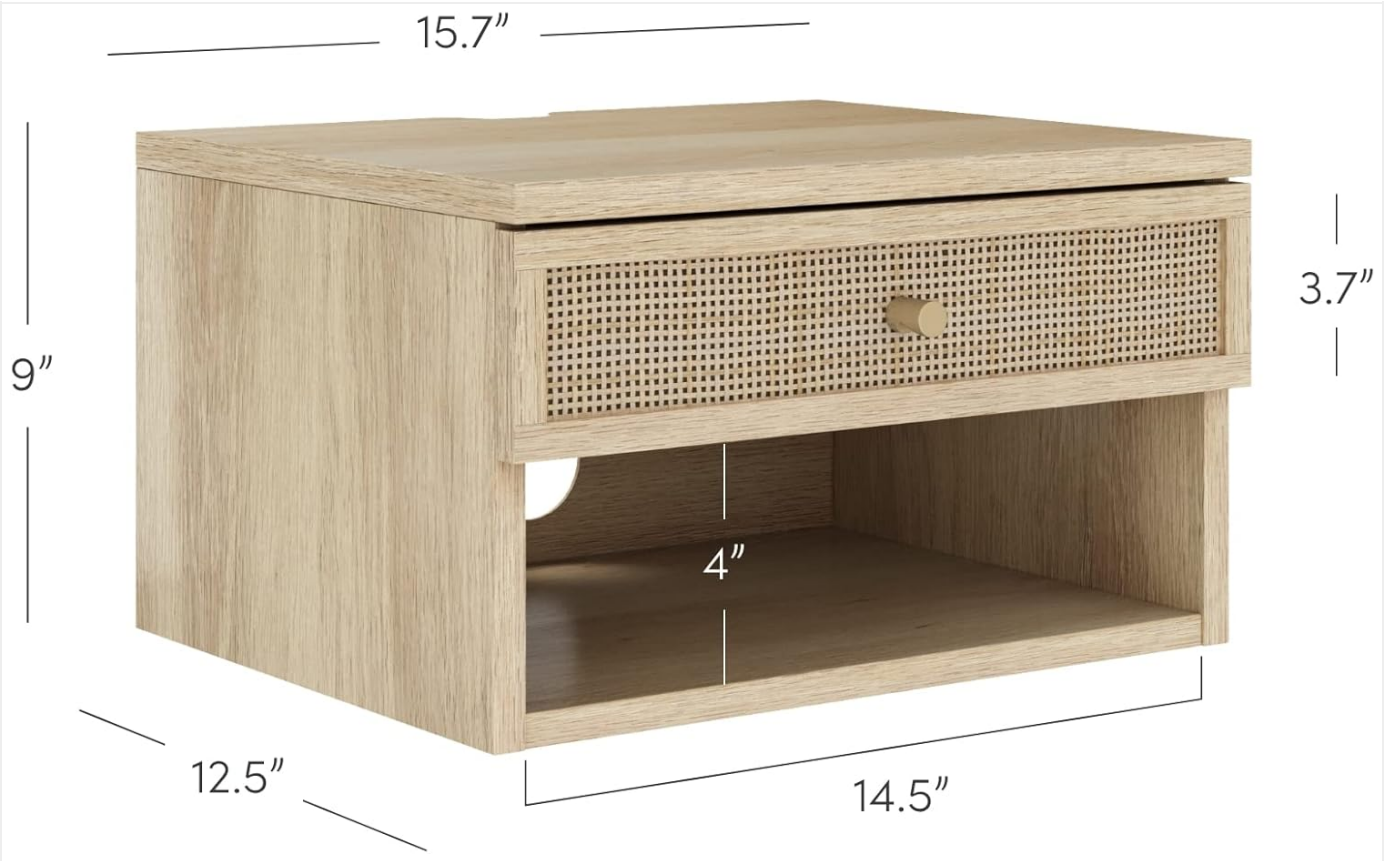
Technical drawing of the Jackson floating nightstand with detailed dimensions: 15.7 inches width, 9 inches height, 12.5 inches depth, 3.7 inches drawer height, and 4 inches open cubby height.
