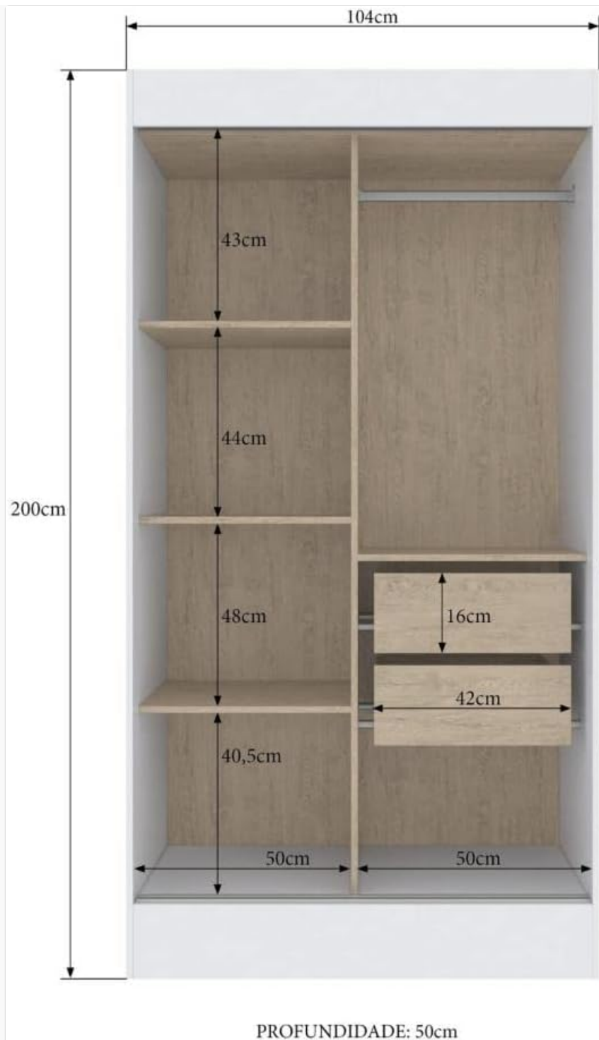
Image 4.2: Technical diagram illustrating the dimensions of the Doripel Lyon Single Wardrobe. The overall height is 200cm, width 104cm, and depth 50cm. Internal shelf heights and drawer dimensions are also indicated.
