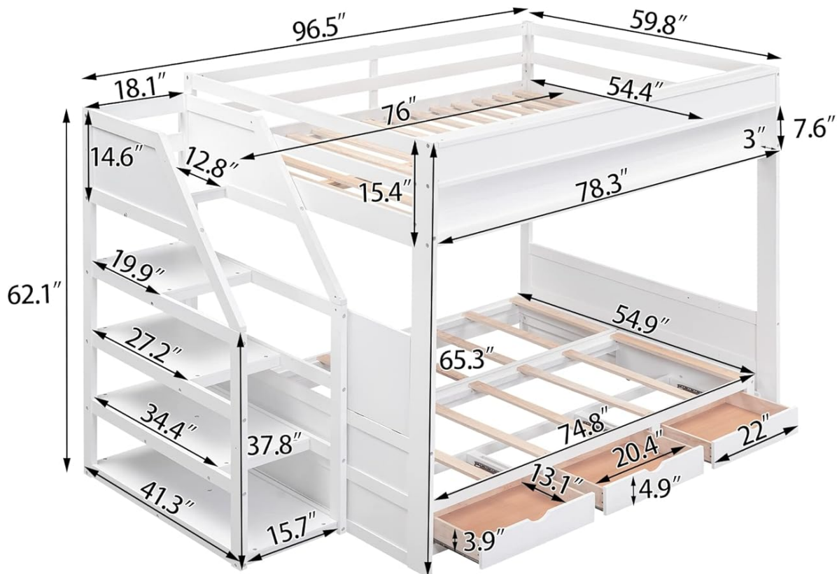
Image: Technical drawing showing all key dimensions of the Polibi Wood Full Size Convertible Bunk Bed in inches.
