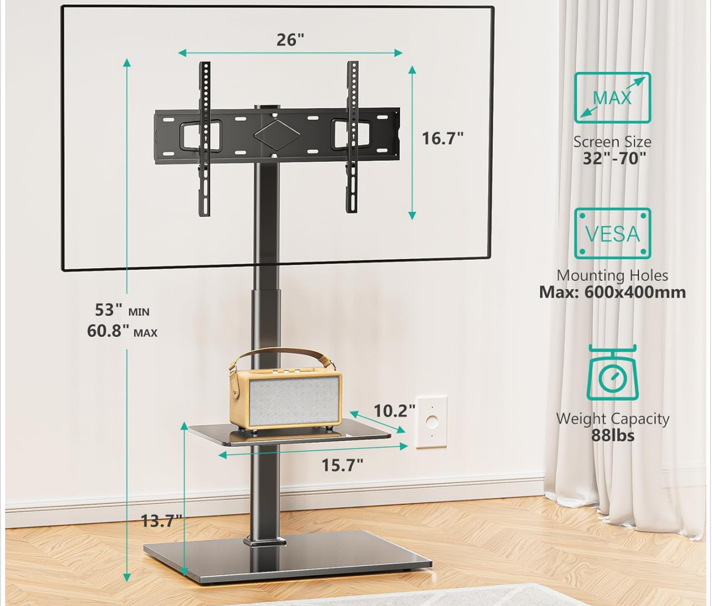
Image: Detailed product dimensions, including overall height (53" min, 60.8" max), shelf height (13.7"), and base dimensions, along with VESA and weight capacity information.
