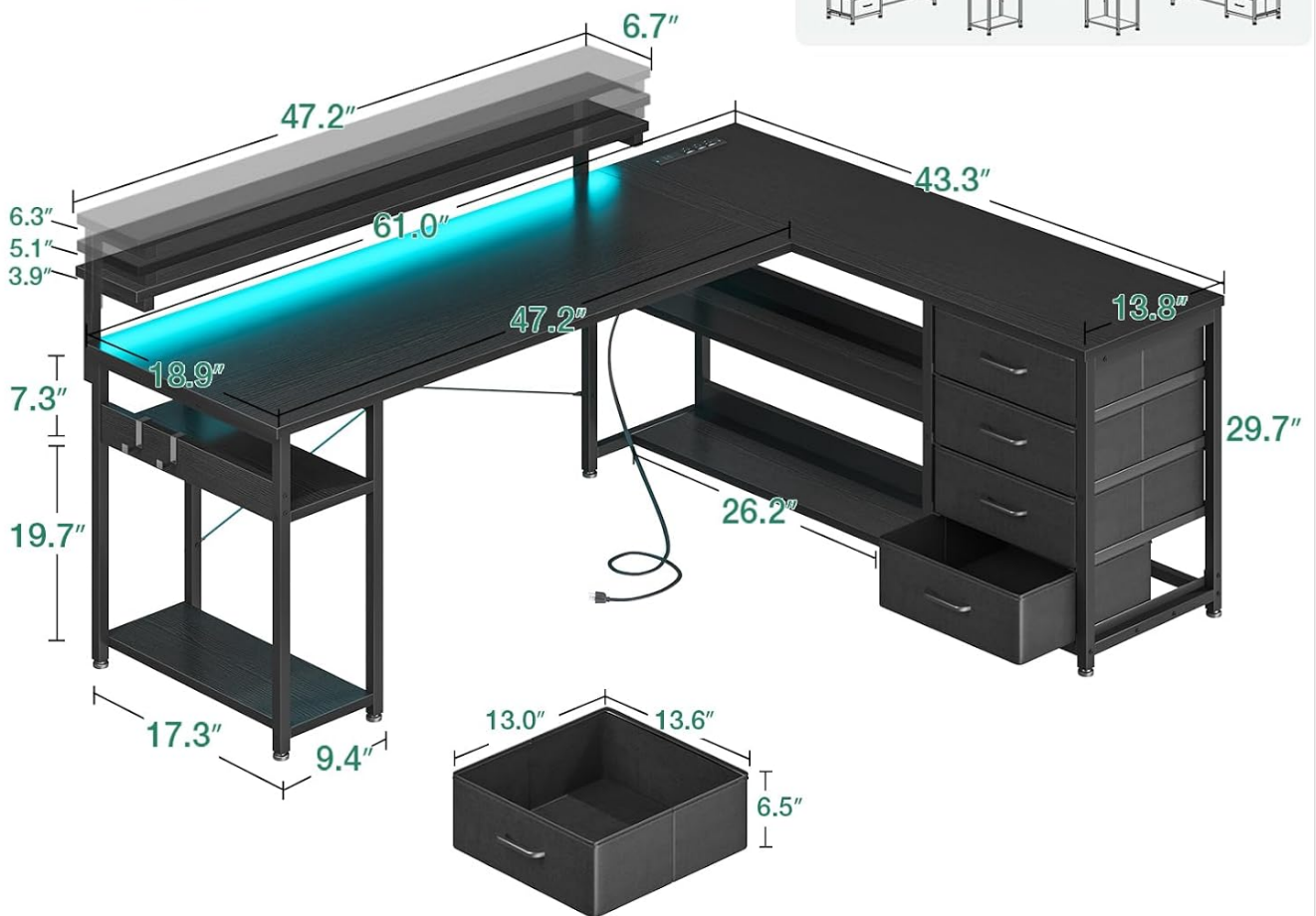
Figure 1: Reversible L-shaped desk configuration and key dimensions. The desk can be assembled with the longer section on either the left or right side to suit your room layout.
