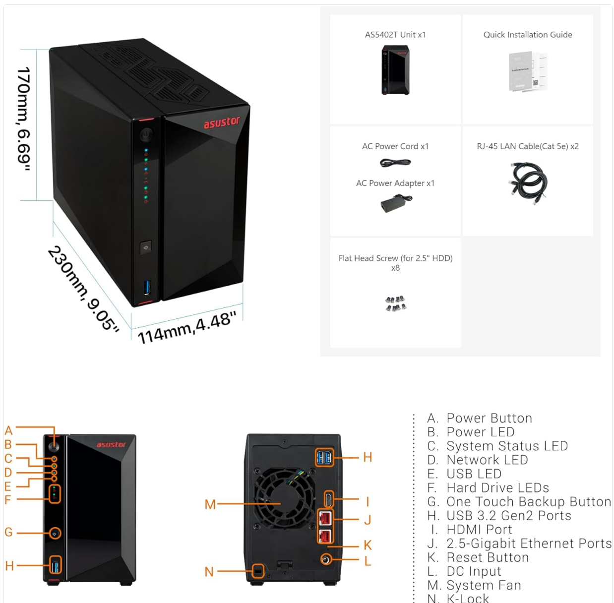
Figure 2: AS5402T Package Contents and Dimensions
