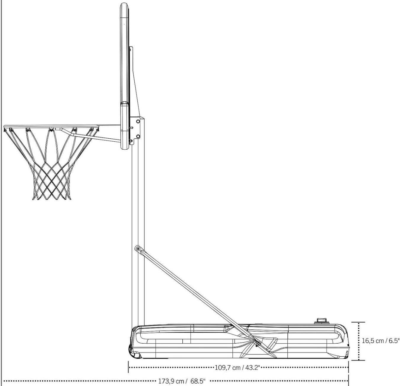
Figure 4: Side View Dimensions.
