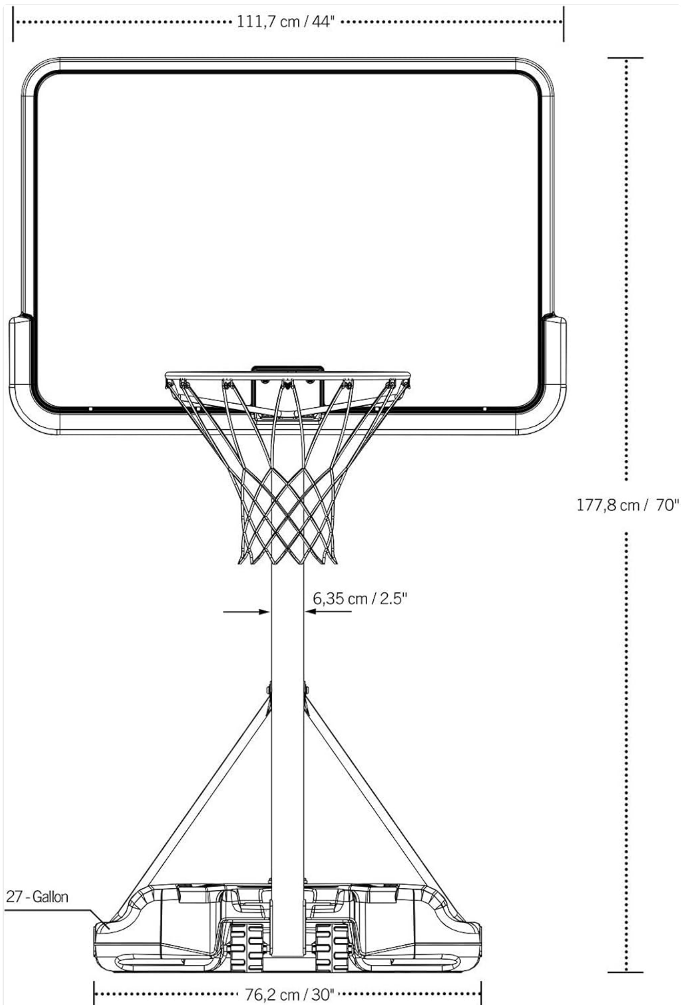
Figure 3: Front View Dimensions.
