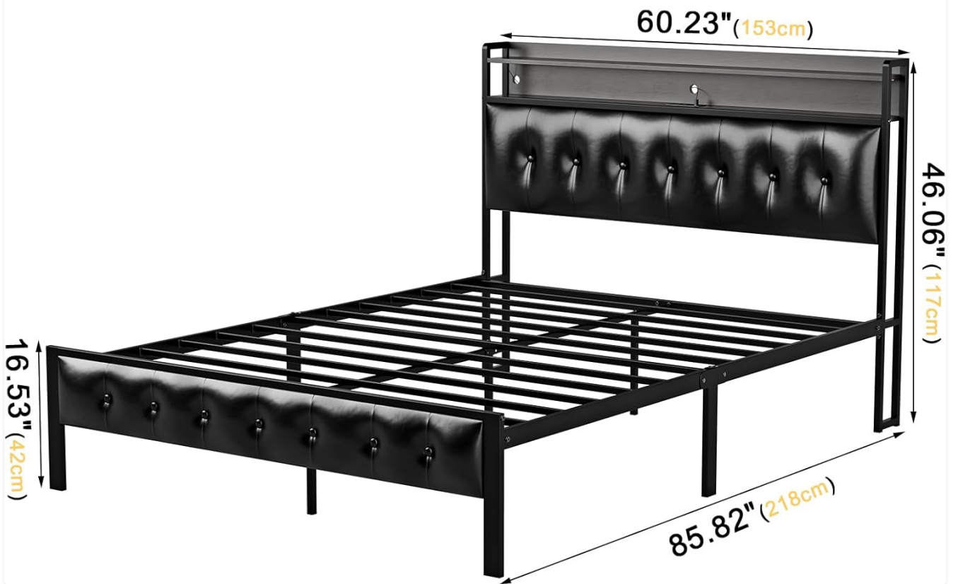
Figure 2: Bed frame dimensions and structural overview.
