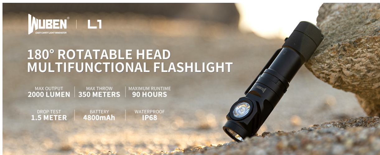
Image 3.1: The WUBEN L1 Flashlight demonstrating its 180-degree rotatable head for flexible lighting angles.
