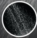
H 2 Ok kinetic Shower
