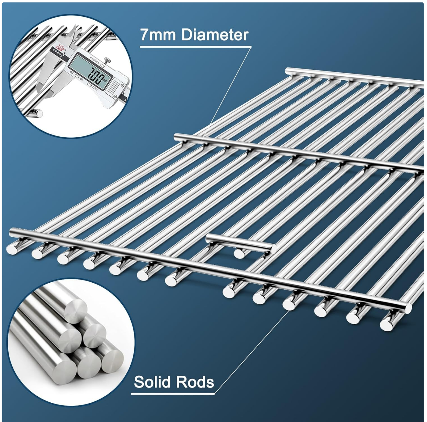
Figure 2: The 7mm diameter of the solid rod bars, indicating enhanced thickness.
