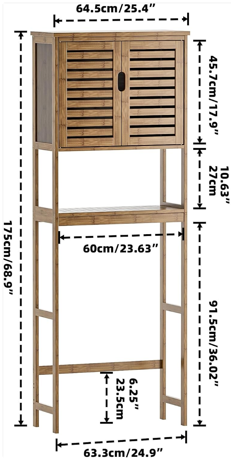
Image: Detailed dimensions of the storage shelf, showing height, width, and depth.
