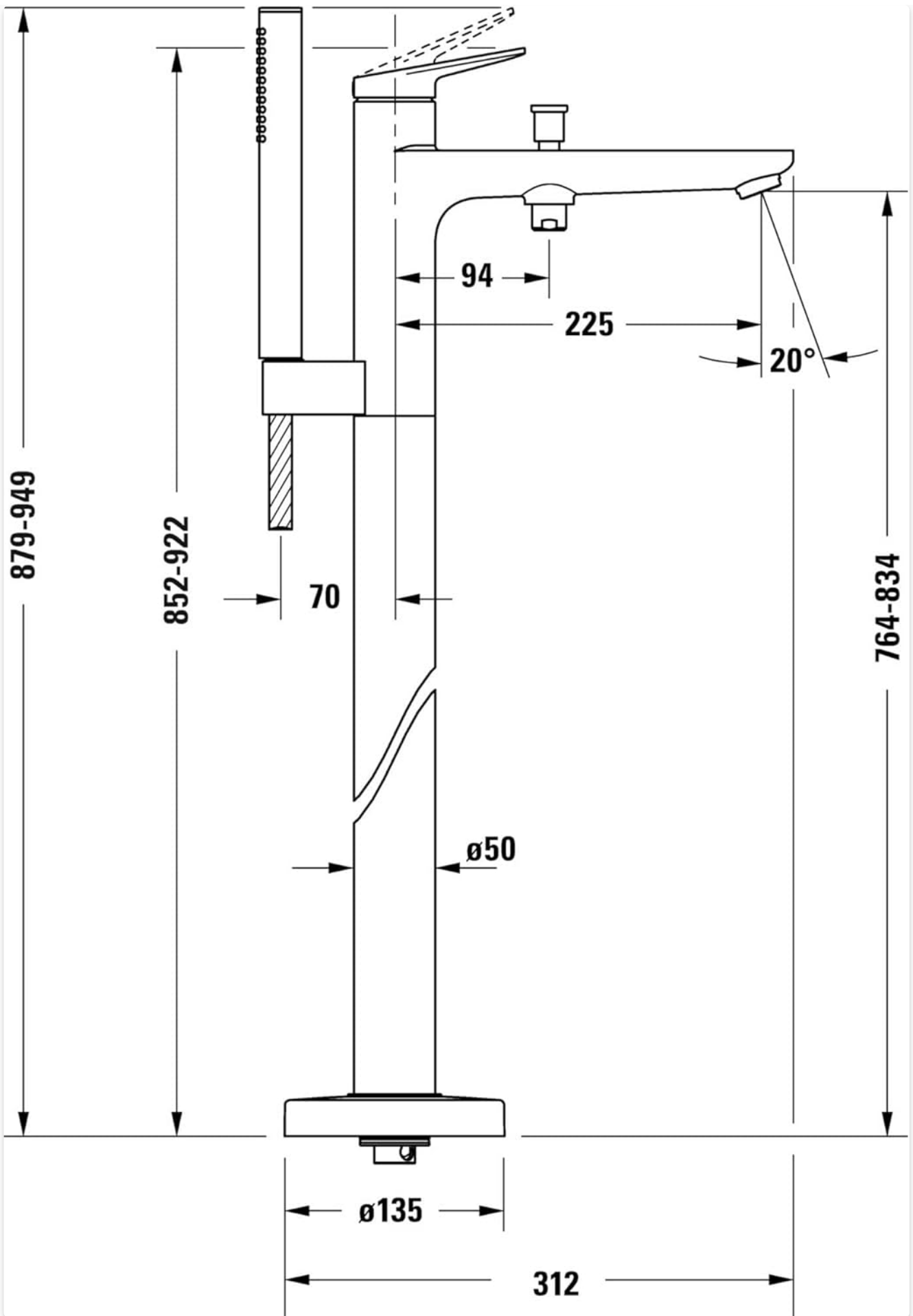
A detailed technical drawing illustrating the front view dimensions of the Duravit Wave freestanding bathtub faucet. Key measurements include overall height, spout reach, and the height of the hand shower holder, providing essential information for installation planning.
