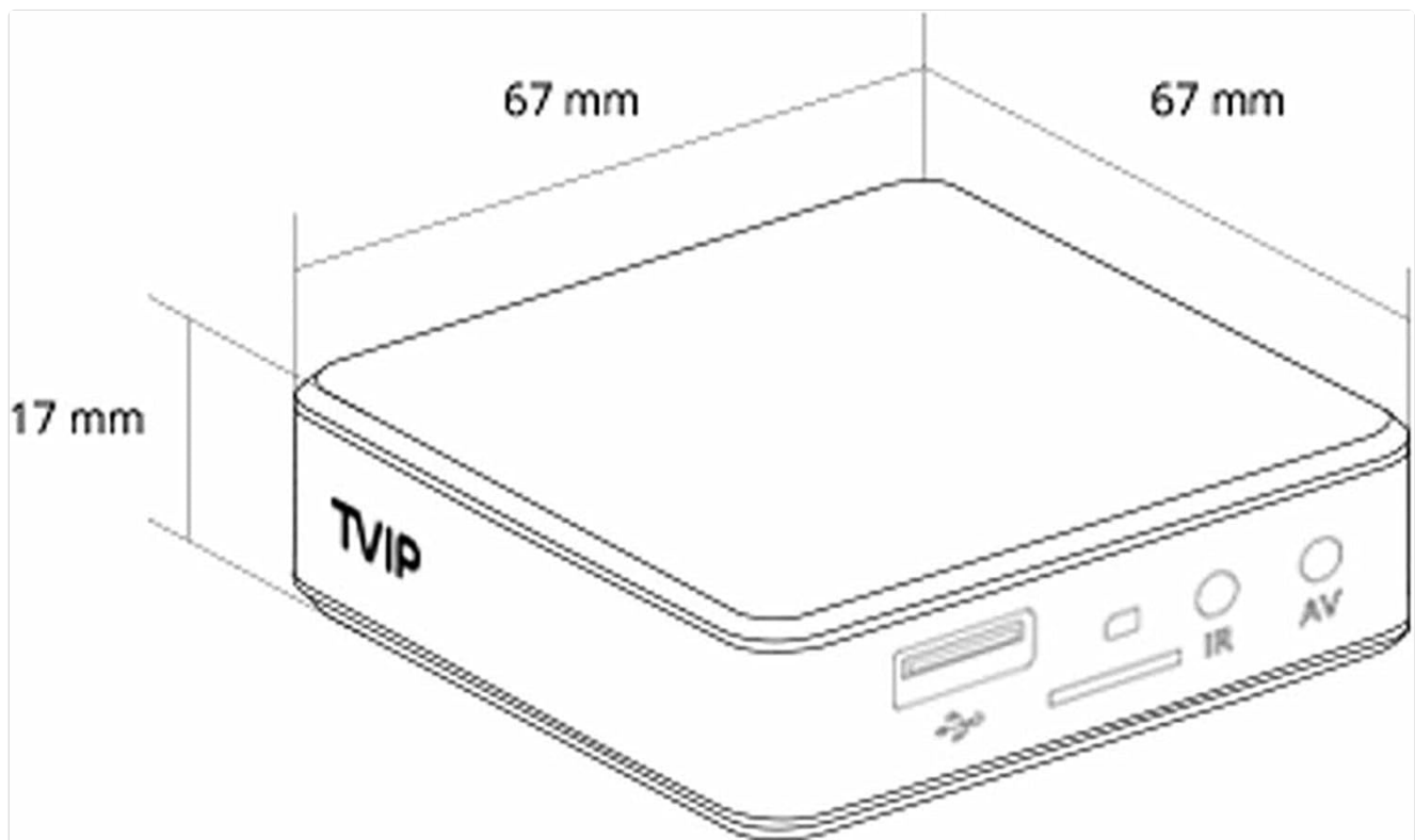
Figure 5: Diagram illustrating the dimensions of the TVIP S-Box v.710 (67mm x 67mm x 17mm).
