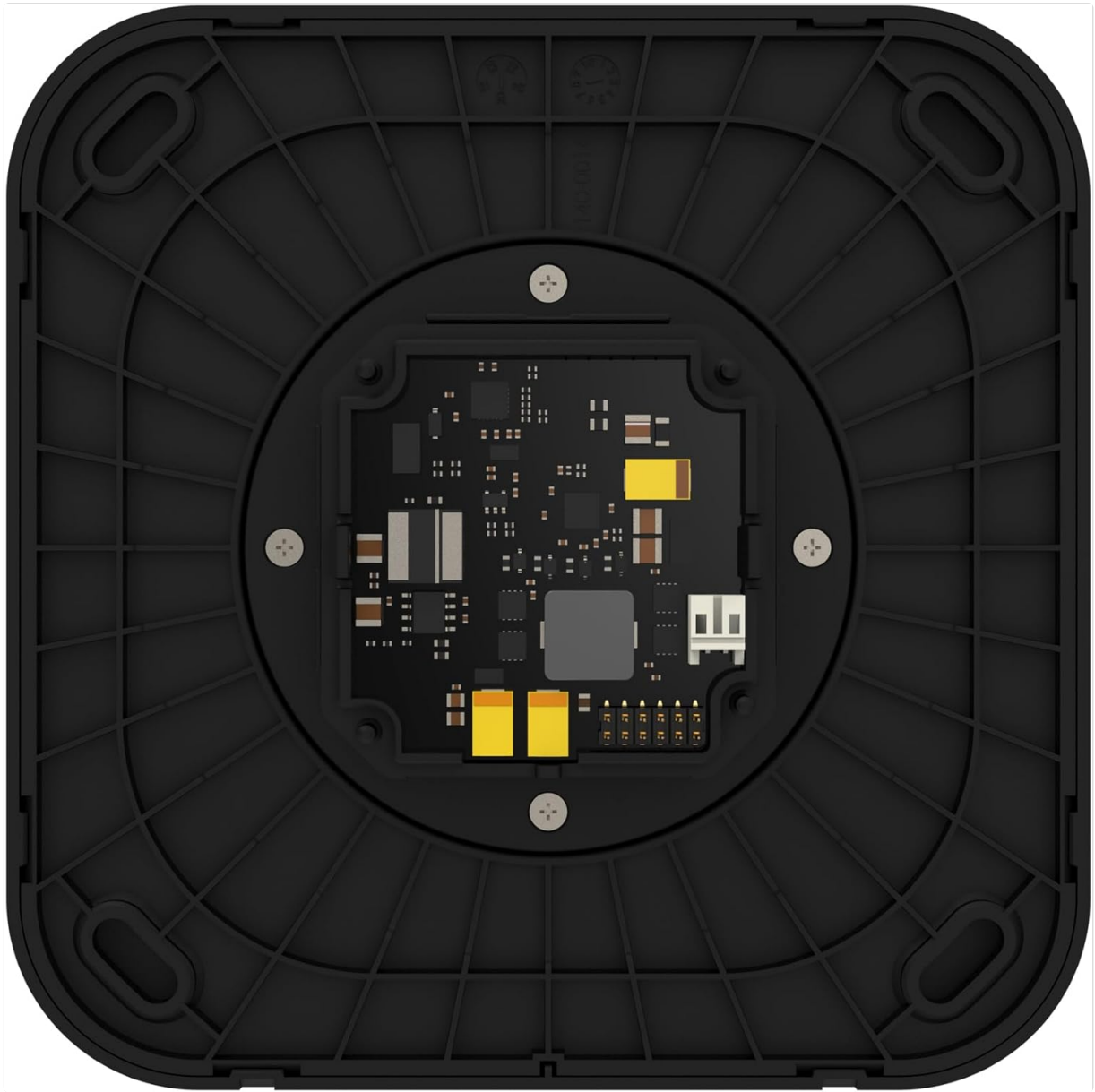
Image: Rear view of the WallStation, showing the internal components and screw holes for mounting.
