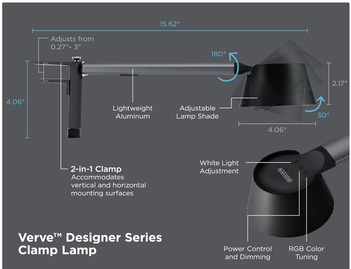
Image: Detailed diagram illustrating the lamp's dimensions and the three touch controls for Power/Dimming, White Light Adjustment, and RGB Color Tuning.
