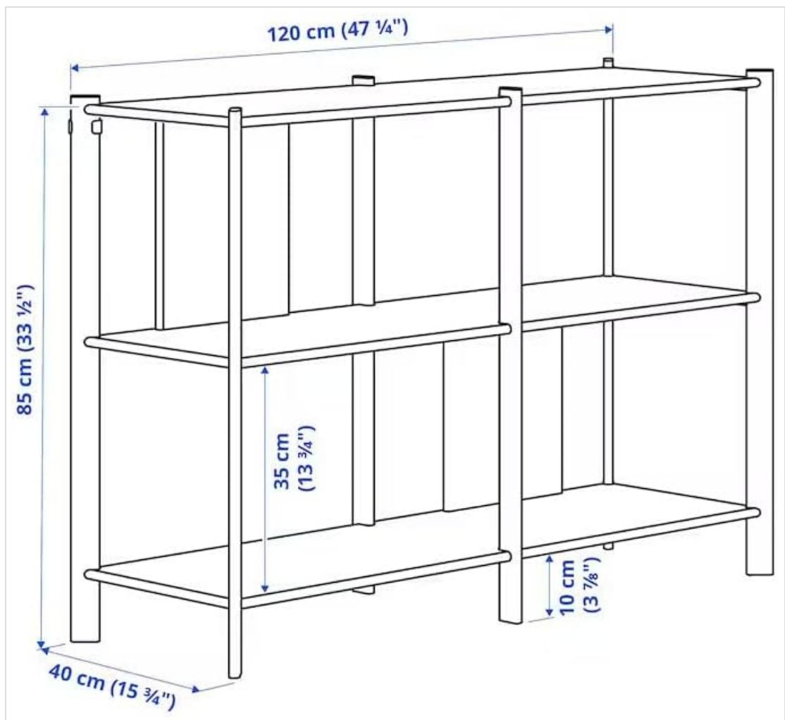
The diagram illustrates the overall dimensions of the JATTESTA shelf unit: 120 cm (47 1/4") width, 40 cm (15 3/4") depth, and 85 cm (33 1/2") height. The spacing between shelves is approximately 35 cm (13 3/4").
