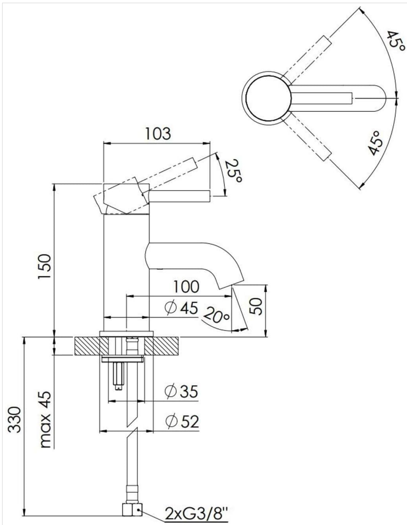
Image: Technical drawing illustrating the dimensions and installation requirements of the Steinberg 100 Series Basin Mixer Faucet, including spout length and overall height.
