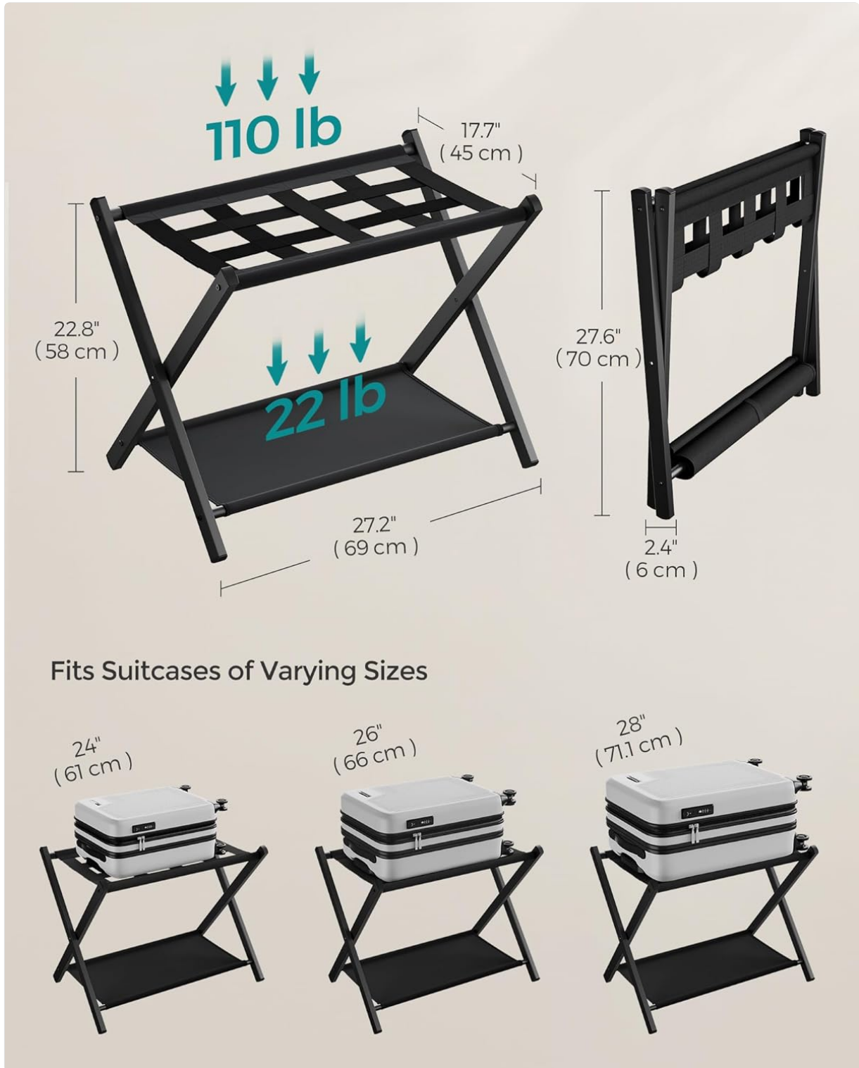
Image: A diagram illustrating the key dimensions (length, width, height, folded size) and maximum load capacities for both the top and bottom shelves of the luggage rack.
