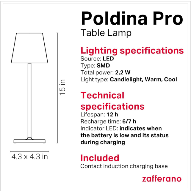
Image: Technical diagram detailing the dimensions and lighting specifications of the Poldina Pro Lamp.
