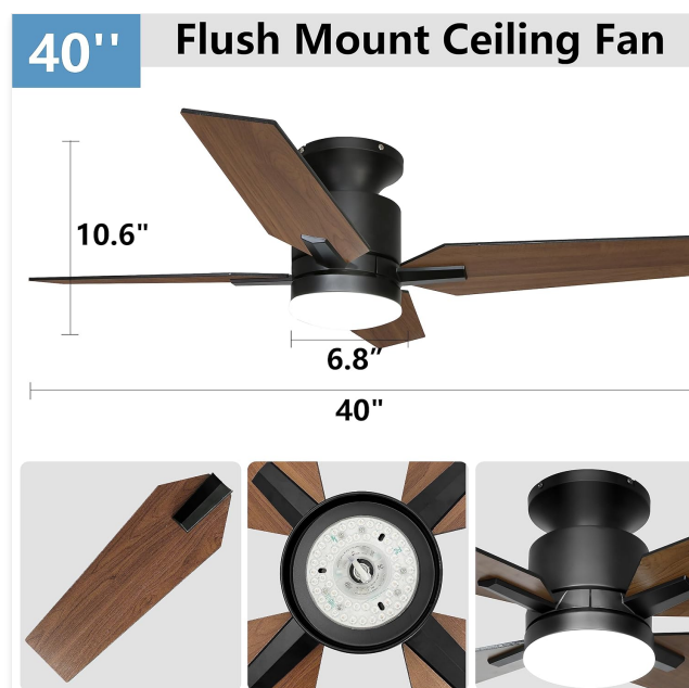
Image 4.1: Fan dimensions for installation planning.
