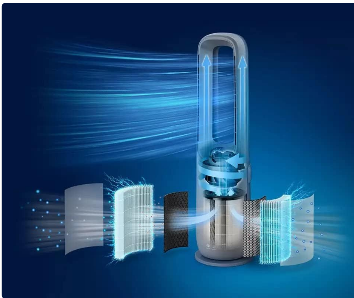
Image: An exploded view showing the multi-layer filtration system of the Philips Air Performer, including HEPA and activated carbon filters.
