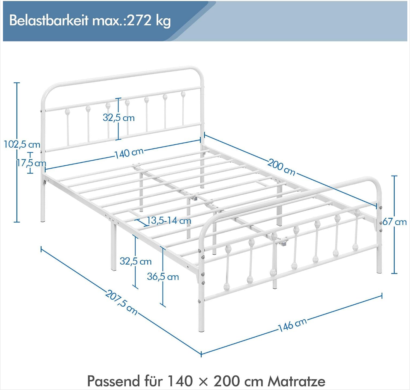
Image: A technical diagram illustrating the key dimensions of the Yaheetech bed frame, including overall length, width, height, headboard height, footboard height, and under-bed clearance.
