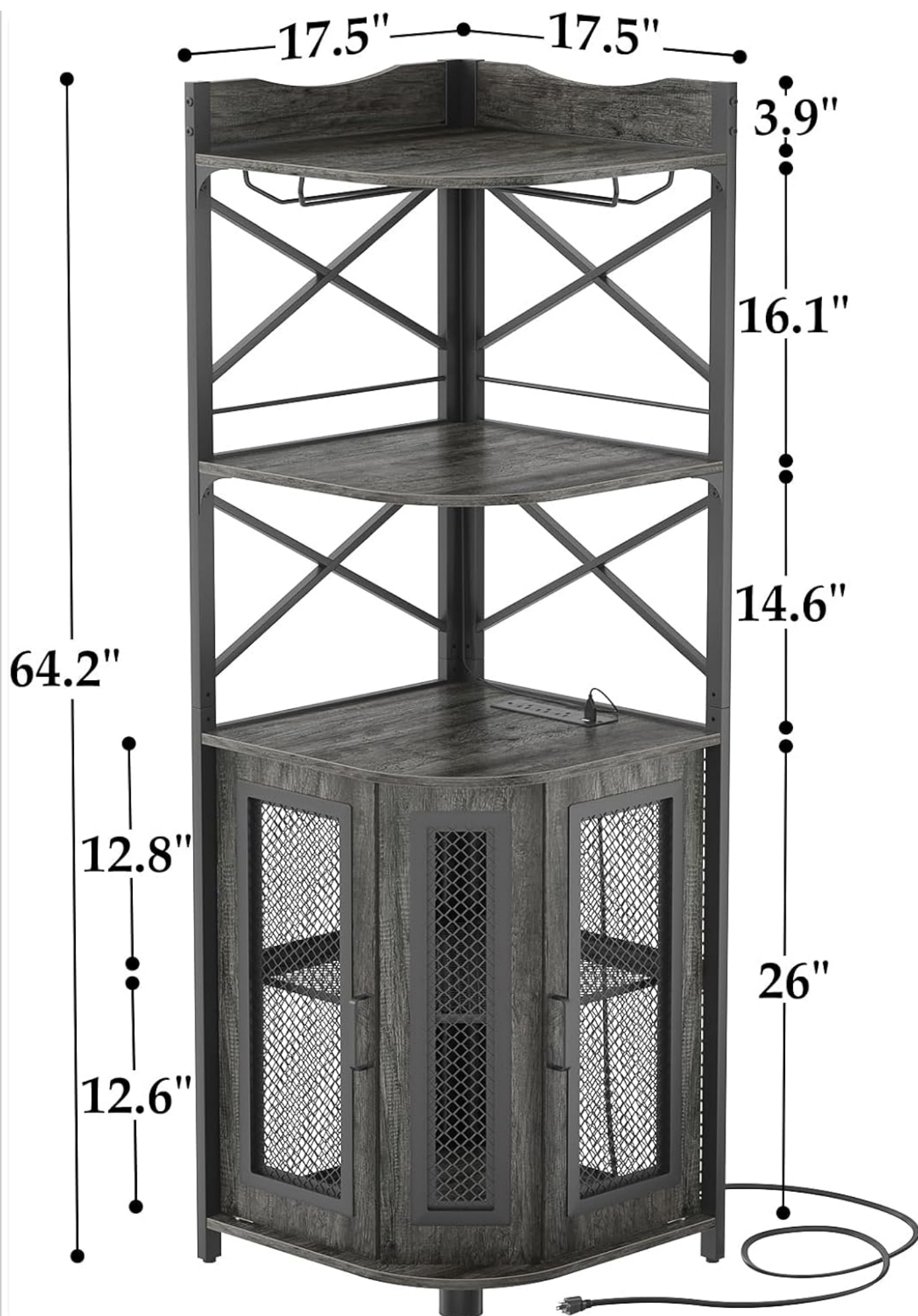
Figure 2: Detailed dimensions of the corner bar cabinet for planning placement.
