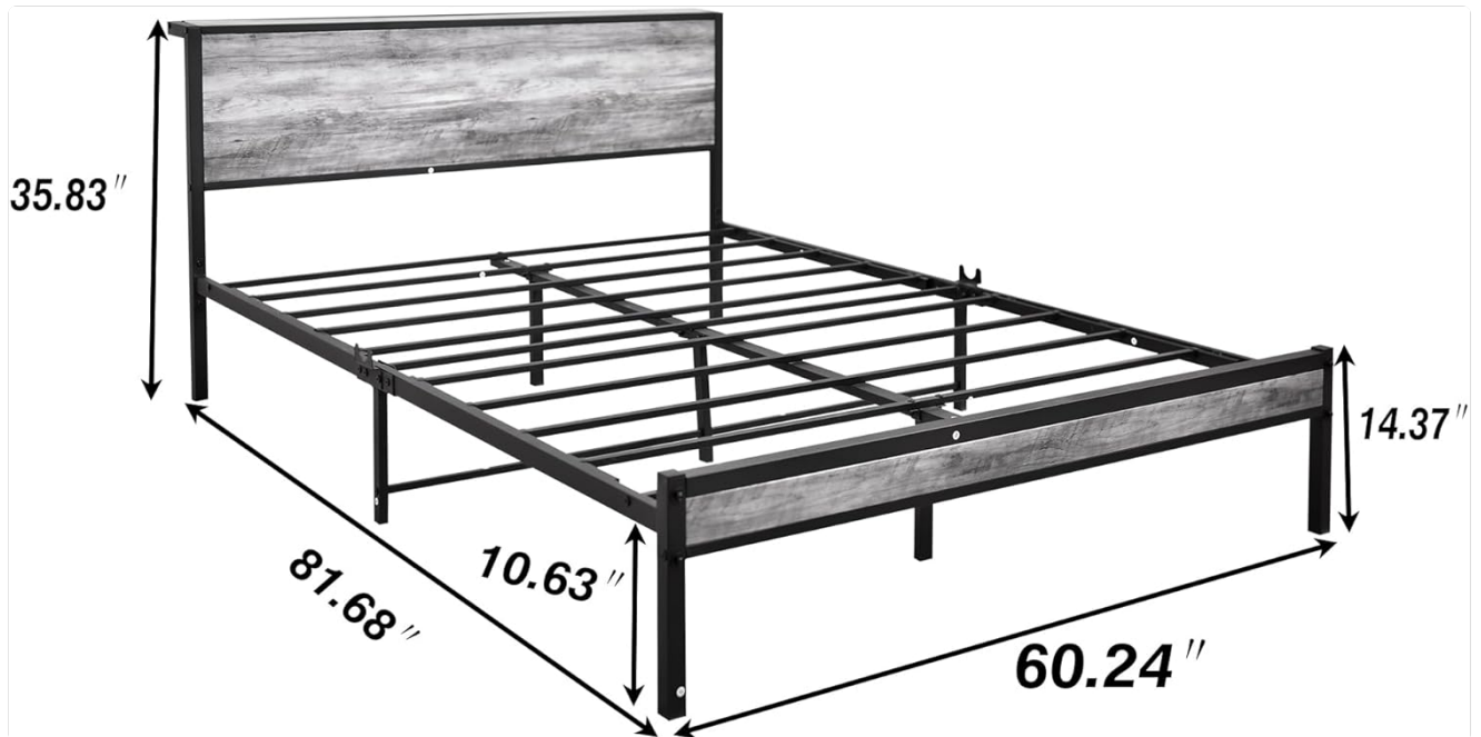
Image: Dimensional diagram of the DUMEE Queen Bed Frame, showing length, width, and height measurements.
