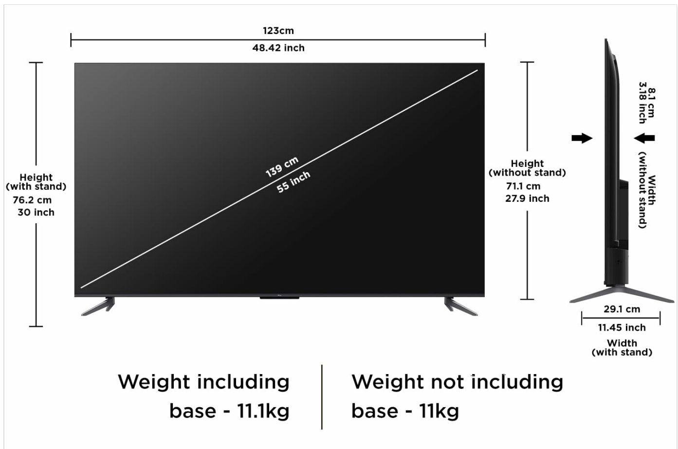
Diagram illustrating the physical dimensions and weight of the TCL 55C645 TV, both with and without the stand.
