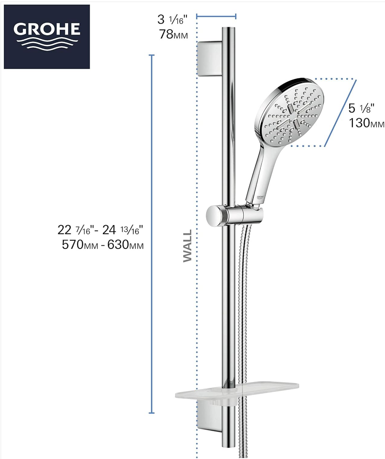
Image: Dimensions of the hand shower and shower bar assembly.
