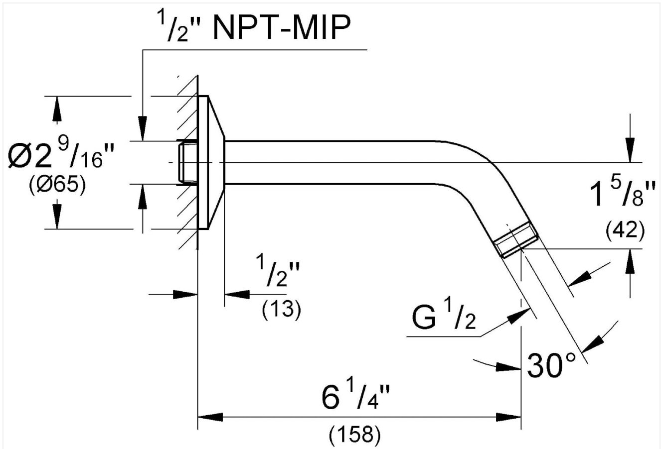
Image: Technical drawing showing the dimensions and installation details of the Relexa 6 1/4" shower arm.
