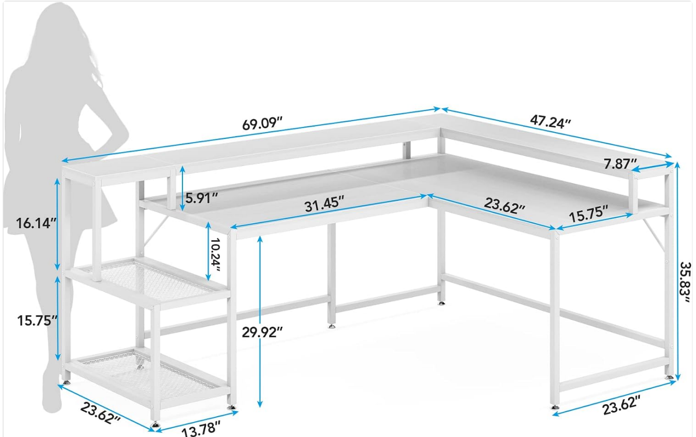
Figure 4.2: Detailed dimensions of the desk, including the monitor stand and storage shelves, to assist with planning and assembly.
