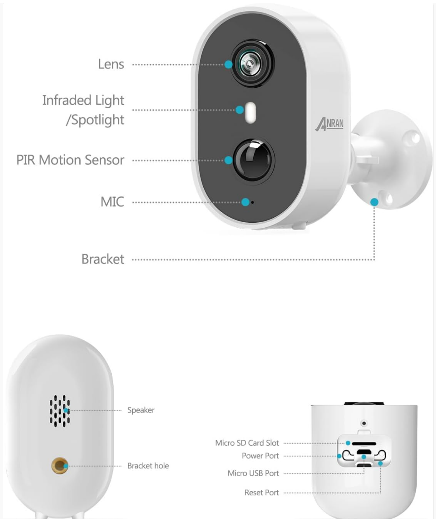
Image: Detailed diagram illustrating the various components of the ANRAN security camera, including the lens, infrared light/spotlight, PIR motion sensor, microphone, speaker, Micro SD card slot, power port, Micro USB port, reset port, and bracket hole.
